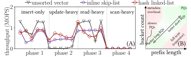
Fig. 1: (A) Dynamic LSM-buffer improves performance by adapting to workload patterns. (B) Hash-hybrid structures provide fine-grained control to tune based on query size.
