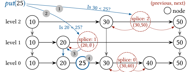
Fig. 2: Splice caches per-level recently accessed nodes, enabling faster traversal for temporal-locality access patterns.
