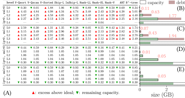
Fig. 15: Prioritizing compactions over writes keeps the LSM-tree in shape and does not accumulate huge compaction debt.
