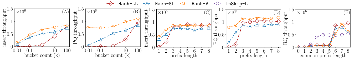
Fig. 10: (A, B) More buckets improve inserts and PQ throughput, adding a minimal per-bucket pointer size overhead. (C, D) Prefix length saturates performance at H = \mathcal{D}^X , whereas (E) RQs throughput is tunable through a common prefix knob.
