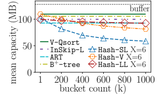
Fig. 13: Increase in bucket count reduces capacity.
