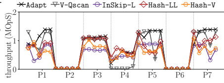
Fig. 20: Adapt benefits from all buffer switching as per workload characteristics
