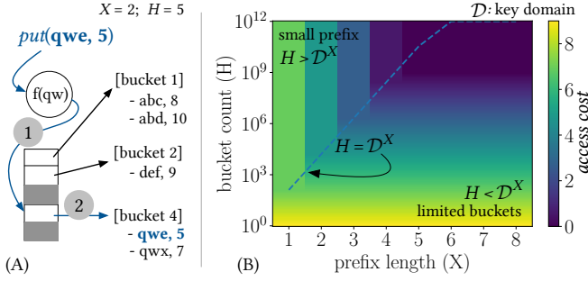
Fig. 3: (A) A flow of hash-hybrid buffer, configured with X = 2 and H = 5 . (B) The higher values of X and H improve performance for put , get , and short-scan operations.
