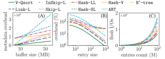
Fig. 4: (A) Metadata overhead is proportional to the #entries in a buffer and (B) entry size, increasing I/Os during (C) flush.
