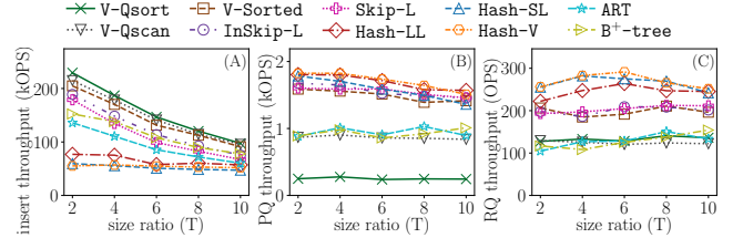
Fig. 17: Throughput drops as the size ratio increases.
