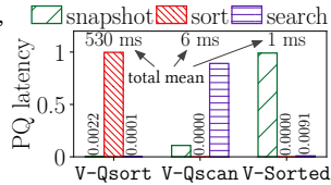
Fig. 12: Sorting and snapshotting slows down V-Qsort
