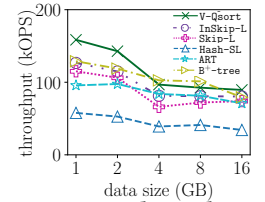
Fig. 19: Throughput scales with data size.
