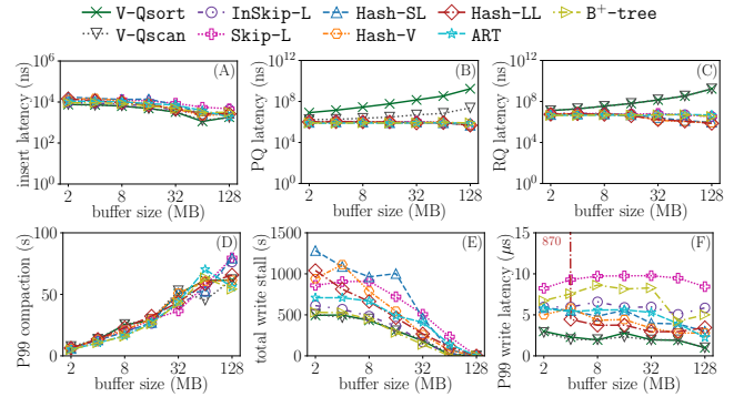
Fig. 16: Except for vector variants, larger buffers improve operational latencies at the cost of high compaction tail latencies. The tail write latency improves as stalls reduce.
