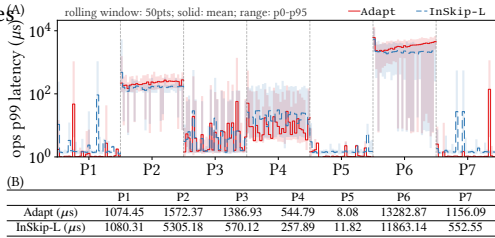
Fig. 21: (A) Adapt buffer adds no extra overhead, as (B) per-phase maximum p99 latency shows no spike with switching.
