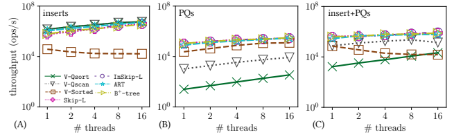
Fig. 18: As the number of threads increases, the throughput improves across buffers for different workloads: (A) write-only, (B) read-only, and (C) mixed workload.
