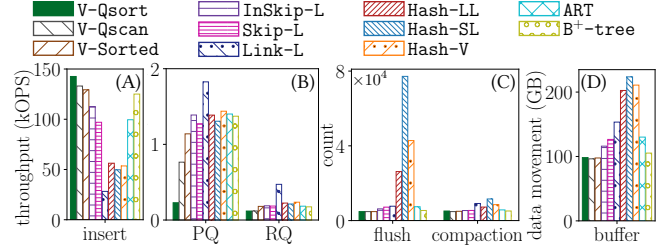
Fig. 5: (A) Vector-variants offer the best throughput for insert-heavy workloads at the (B) cost of slower queries, (C) but perform fewer flushes and (D) less data movement.
