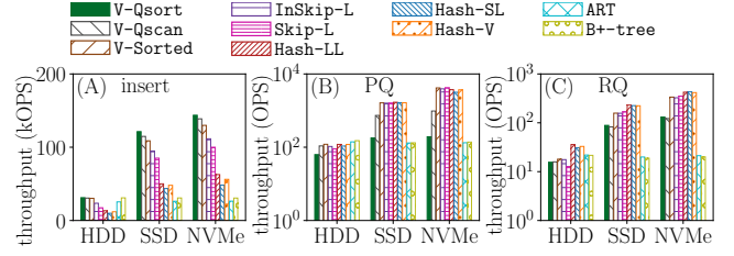
Fig. 22: NVMe consistently outperforms SSD and HDD.
