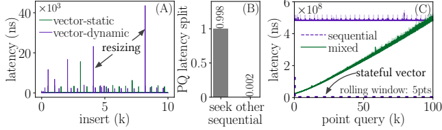
Fig. 11: In V-Qsort, (A) latency spikes due to resizing, and (B, C) sorting slows down PQs significantly for larger buffers.
